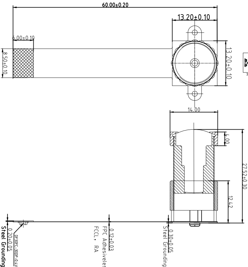
TOP VIEW
